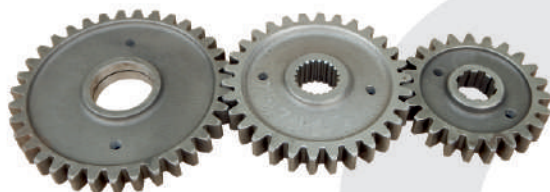
Side Gear Set 35T x 30T x 23T Part No. NR 3121
