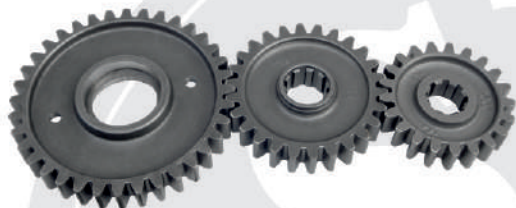
Side Gear Set (36Tx26Tx21T) Part No. NR 1517
