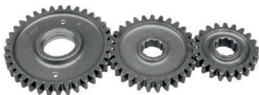
Side Gear Set 36Tx29Tx21T Part No. NR 308
