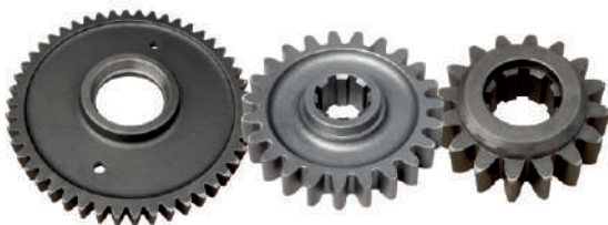
Gear Set 16Tx48Tx23T Part No. NR 1565
