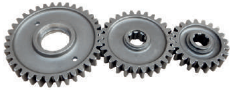
Side Gear Set 21Tx28Tx36T Part No. NR 1745
