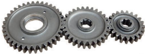
Side Gear Set 36Tx28Tx21T Part No. NR 206
