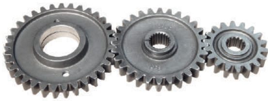
Side Gear Set 33T x 28T x 18T Part No. NR 626
