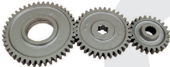
Side Gear 43Tx34Tx24T Part No. NR 2730
