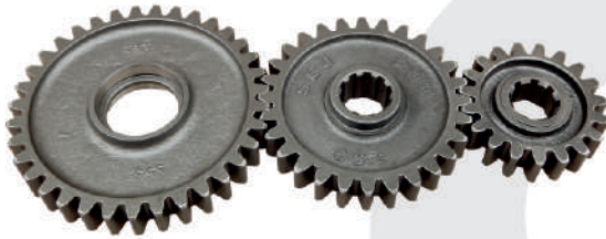
Side Gear 35Tx28Tx19T Part No. NR 1002
