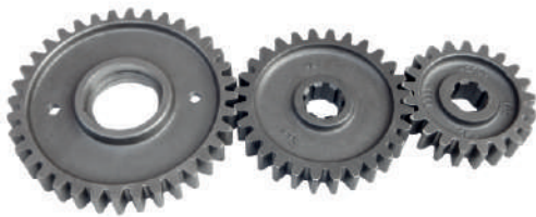
Side Gear Set 21Tx26Tx36T Part No. NR 1006
