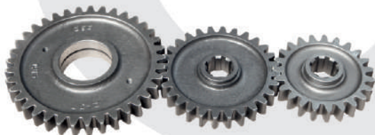
Side Gear Set 37T x 28T x 23T Part No. NR 202
